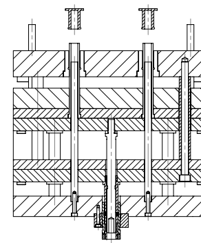
SECTION D-D SECOND EJECTOR STROKE
