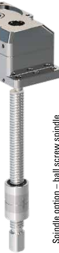
Standard – ball screw spindle Pitch 5mm – stroke 150mm
